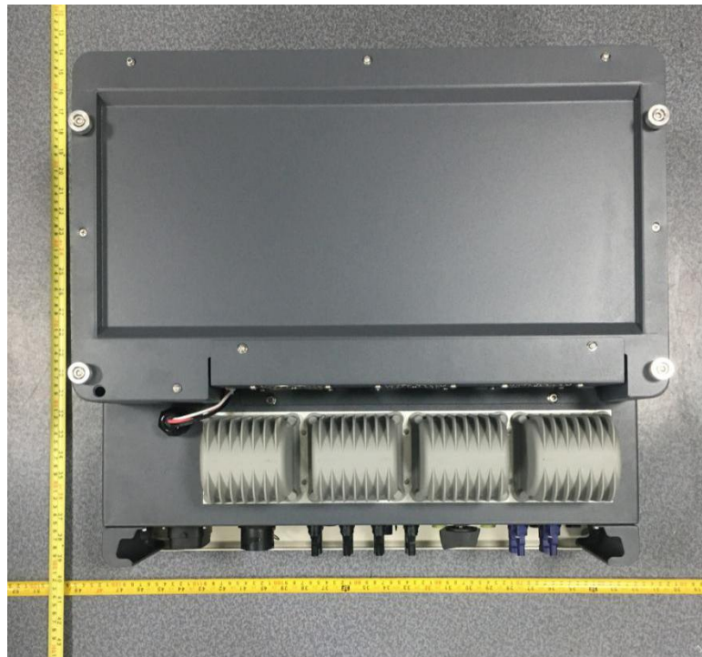
Fig. 2 (HYD 10-20KTL-3PH Back of the body)
