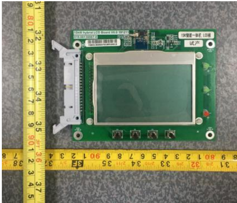
Fig. 10 (HYD 10-20KTL-3PH Front of the display)
