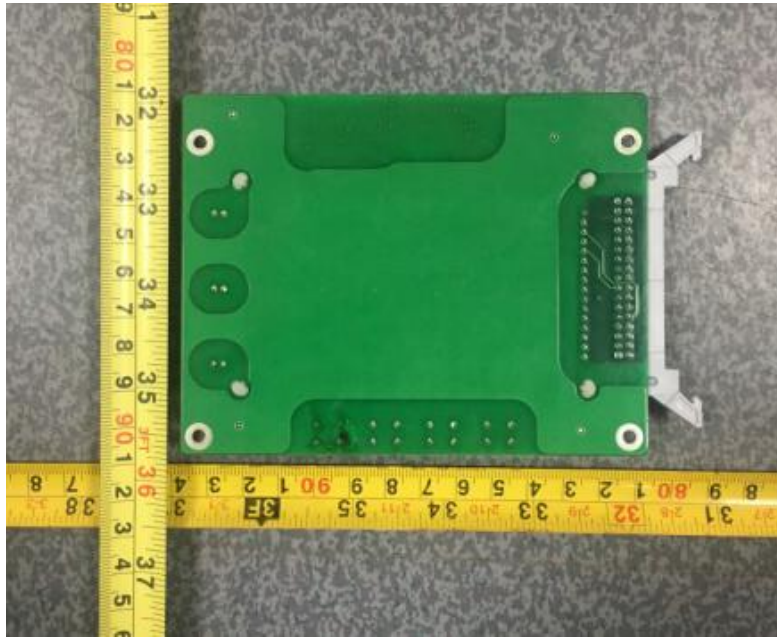
Fig. 11 (HYD 10-20KTL-3PH Back of the display)
