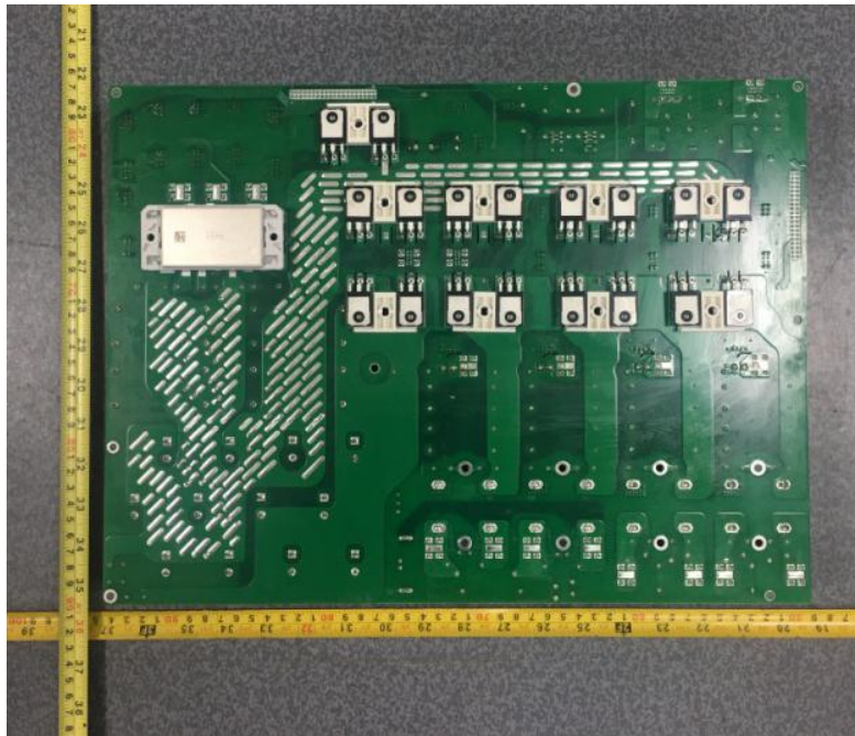
Fig. 5 (HYD 10-20KTL-3PH Power board back)
