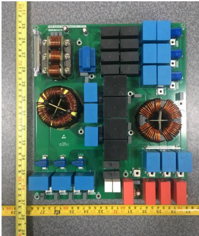
Fig. 6 (HYD 10-20KTL-3PH Output board front)
