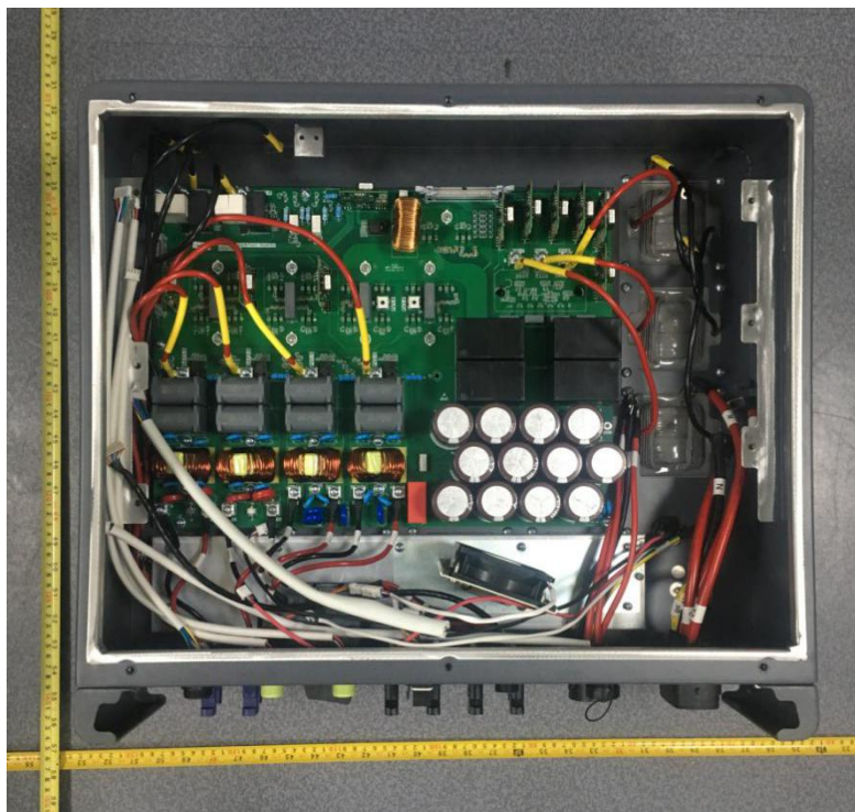
Fig. 14 (HYD 10-20KTL-3PH Bottom of the machine)
