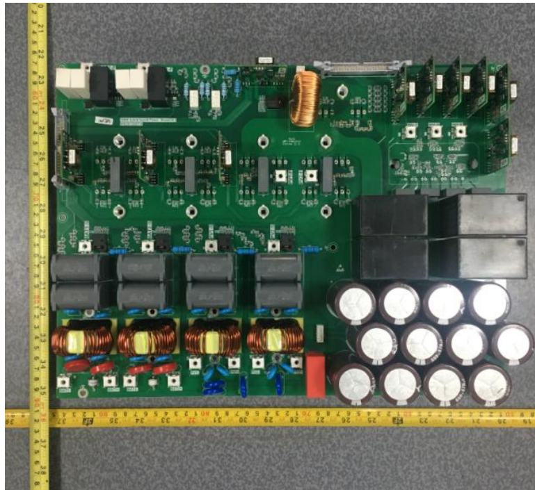
Fig. 4 (HYD 10-20KTL-3PH Power board front)
