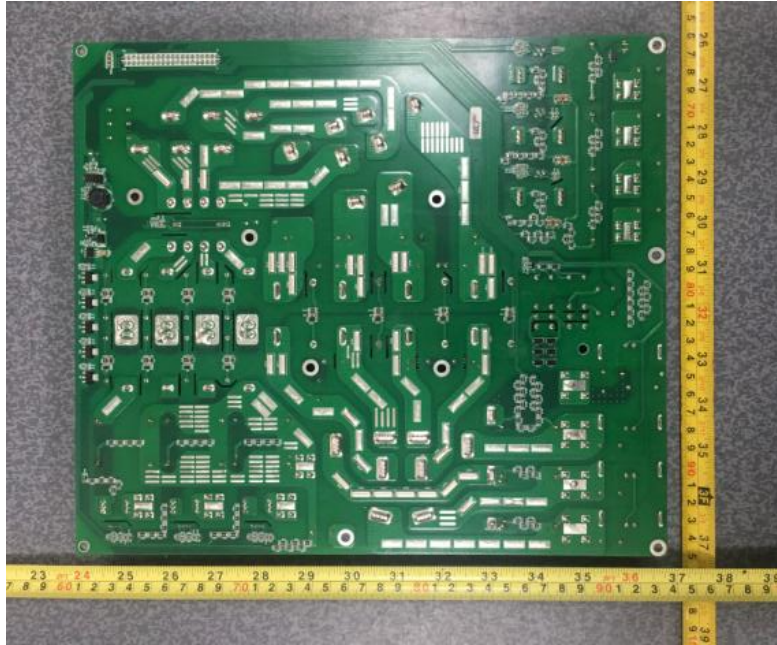
Fig. 7 (HYD 10-20KTL-3PH Output board back)
